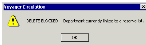
Figure 8-75. Delete Blocked
