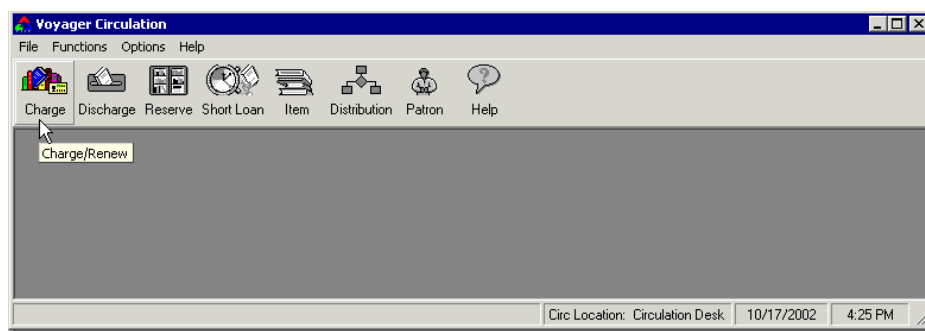
Figure 6-7. Charge Button
