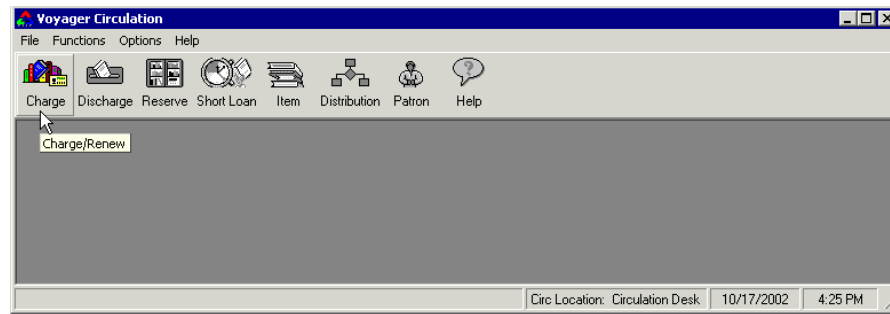
Figure 4-105. Charge Button
