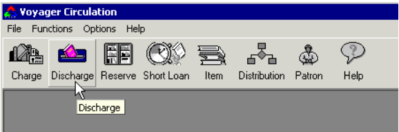
Figure 7-4. Discharge Button
