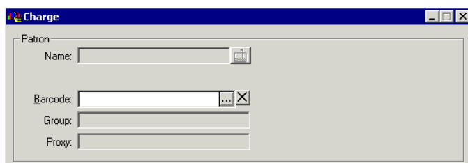
Figure 3-7. Charge Workspace
