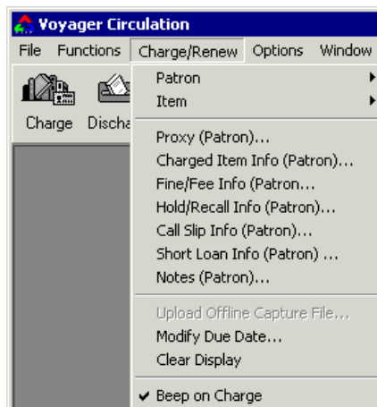
Figure 14-5. Charge/Renew Menu
