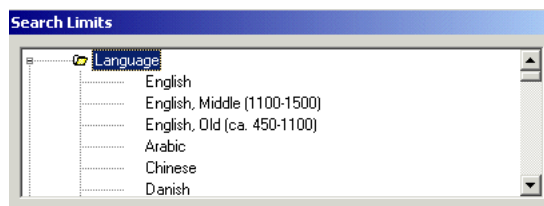
Figure 3-52. Language limits
