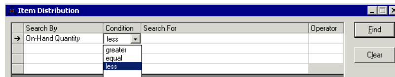
Figure 11-5. Condition Menu
