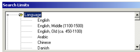
Figure 3-67. Language limits
