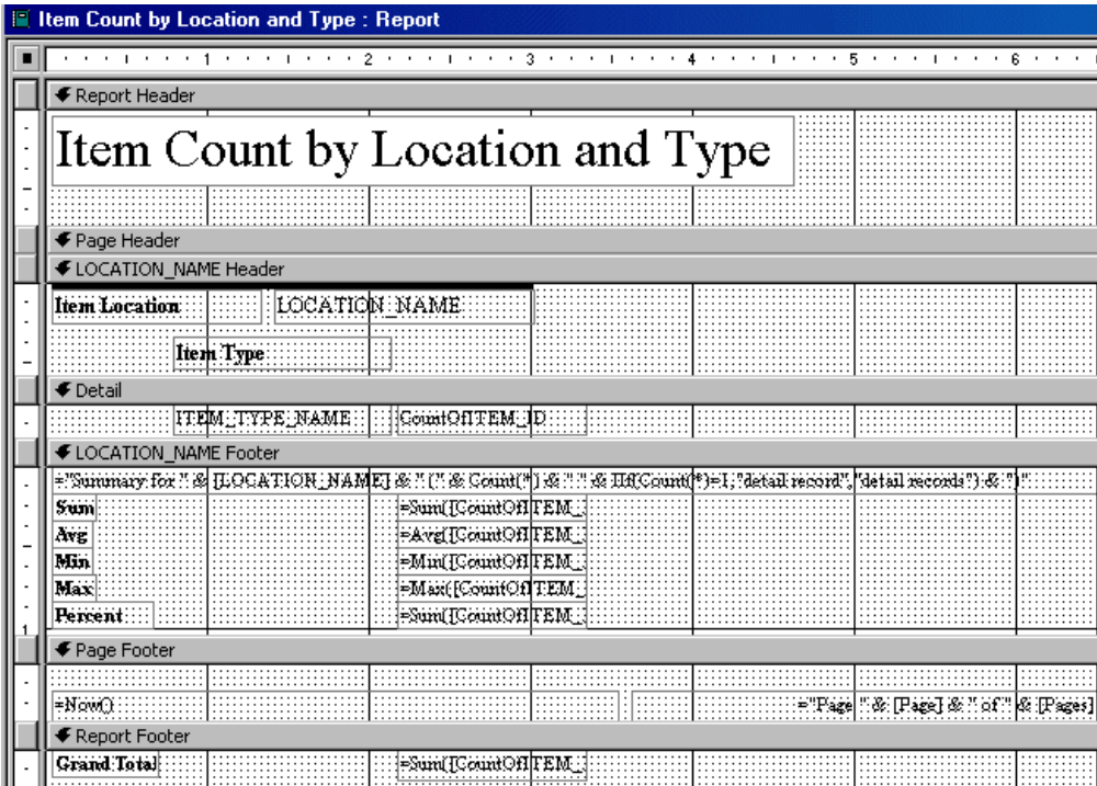
Figure 7-4. Designing the Item Count by Location and Type report in Access
