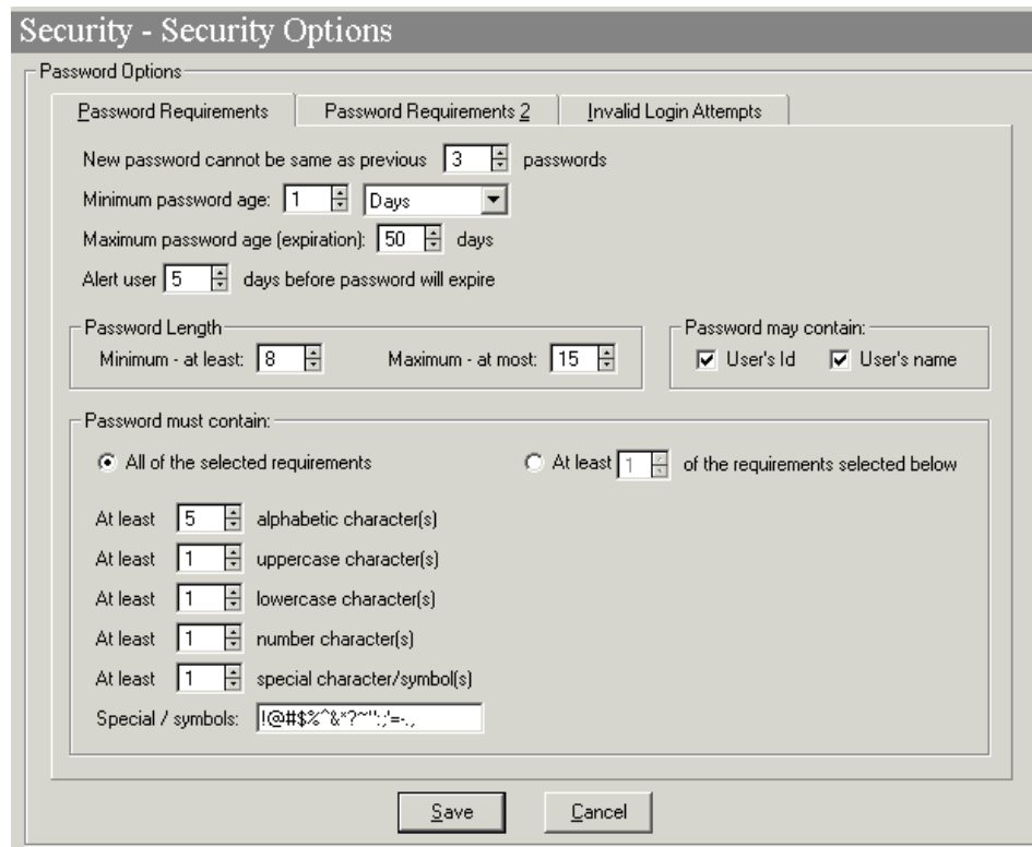
Figure 9-87. Security - Security Options (Password Requirements Tab)
