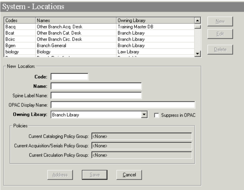
Figure 10-28. New Location section
