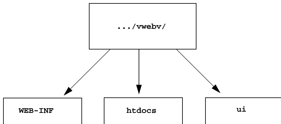
Figure 3-1. .../vwebv/ directory
