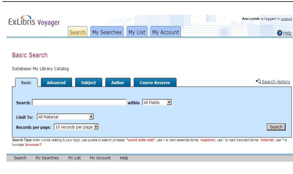
Figure 2-7. Basic Search
