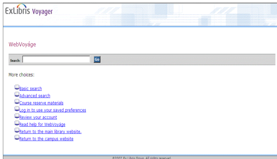
Figure 3-5. Default window
